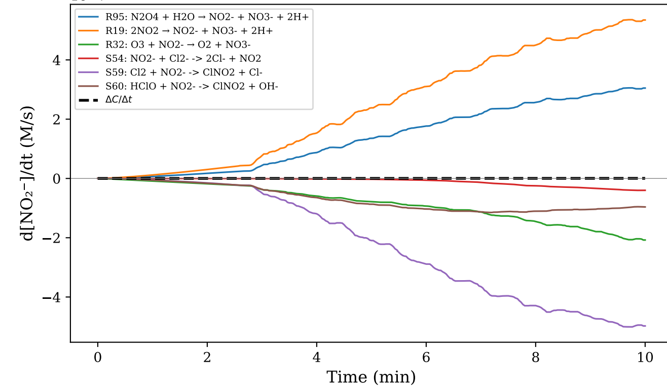
(c) \text{NO}_2^-
